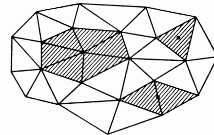
Fig 3.8 The support of different basis functions.
