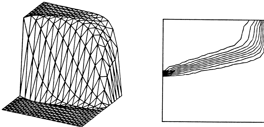
Fig 9.7 Solution graph and level curves for streamline diffusion method for problem in Example 9.2 (a) without and (b) with shock-capturing
