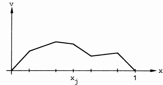
Fig 1.3 Example of a function v \in V_h
