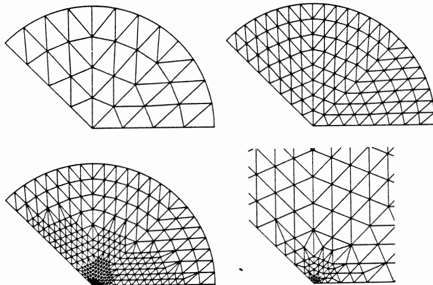
Fig 4.2 Sequence of meshes obtained by adaptive FEM
