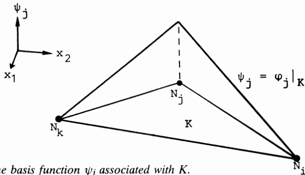
Fig 1.12 The basis function \psi_j associated with K .
