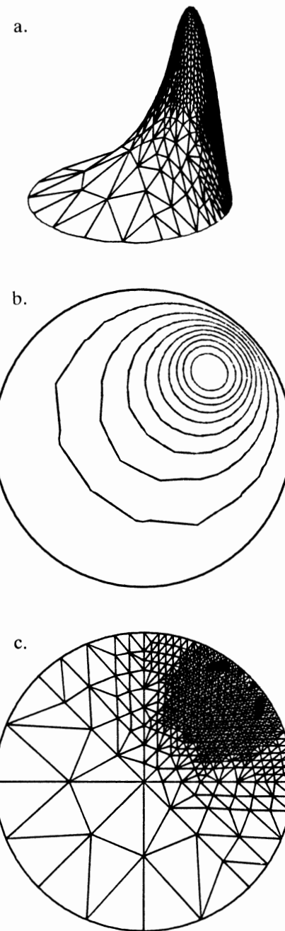
Fig 1.16 Solution graph (a), level curves (b) and triangulation (c) for finite element method for Dirichlet problem.
