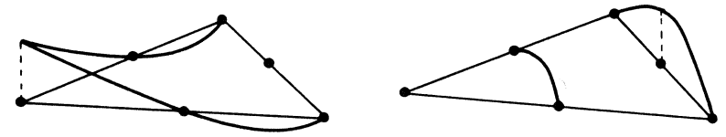
Fig 3.3 Different basis functions for P_2(K)
