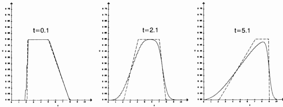
d. Lax-Friedrichs' method.
