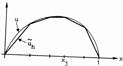
Fig 1.6 The interpolant \tilde{u}_h .
