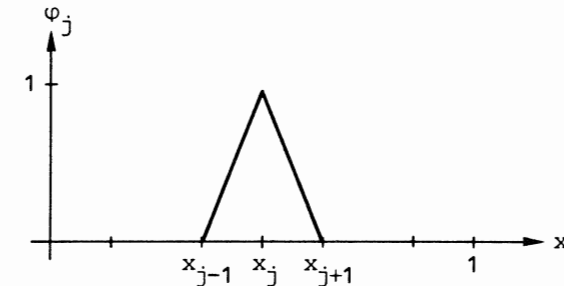
Fig 1.4 The basis function \varphi_j
