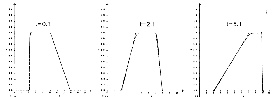
b. Streamline diffusion method with shock-capturing, \bar{\delta}=\delta=h=0.1 .
