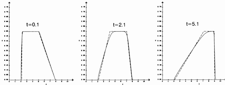
e. Goudonov's method.
