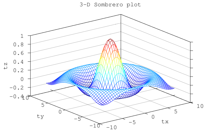
Figure 15.5: Mesh plot.
