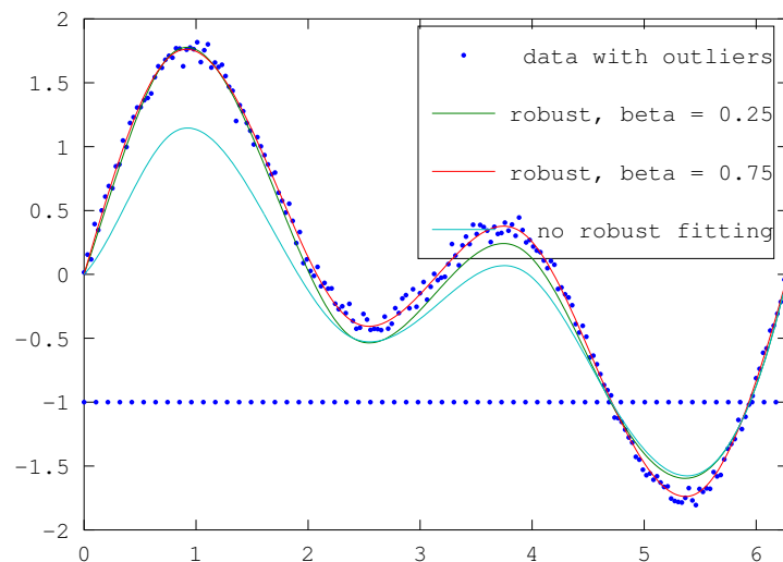
Figure 28.5: Comparison of two different levels of robust fitting ( \beta = 0.25 and 0.75 ) to noisy data combined with outlying data. A conventional fit, without robust fitting ( \beta = 0 ) is also included.
